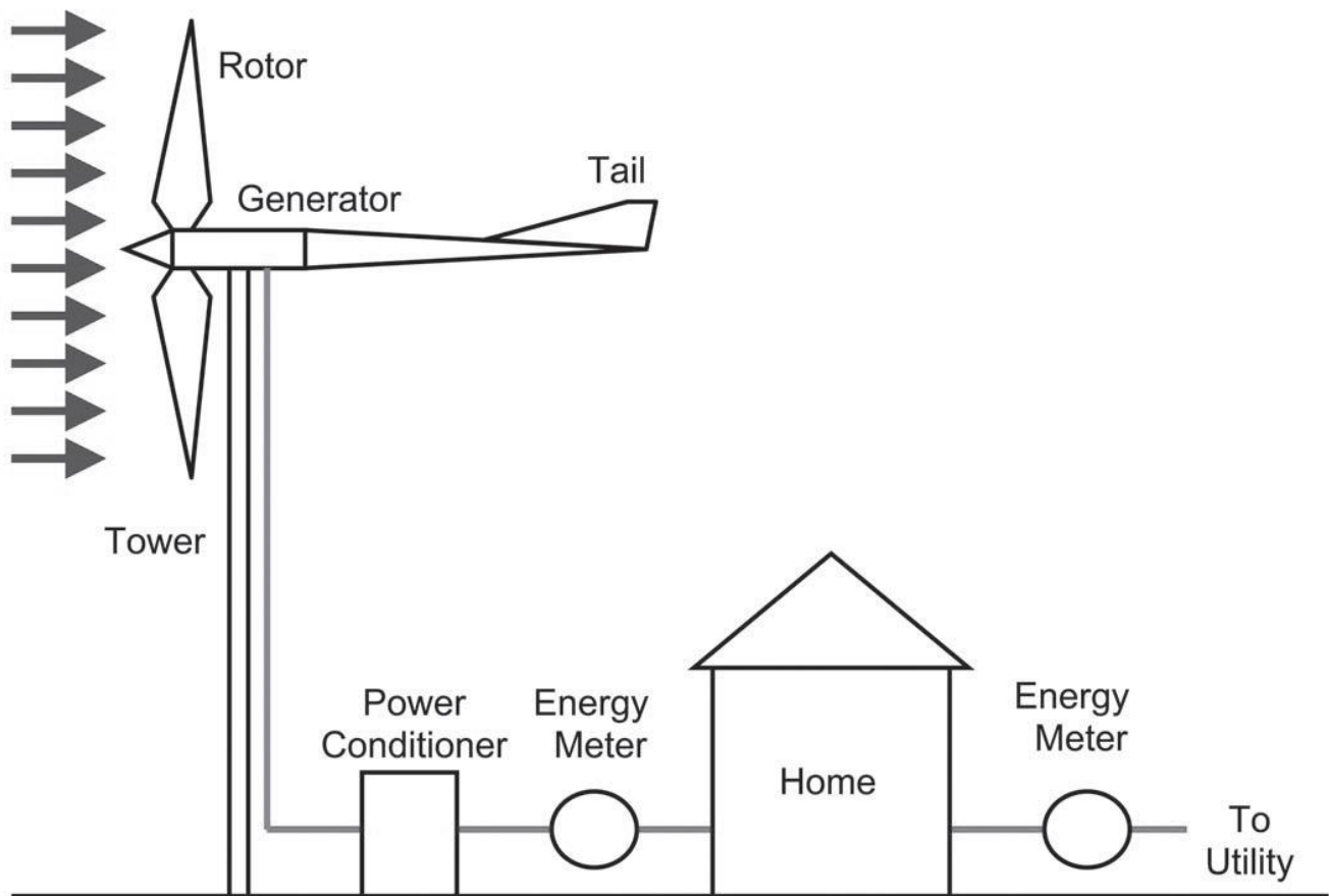
Figure - Grid-connected residential wind energy system. Meter between power conditioner and home is Optional.
