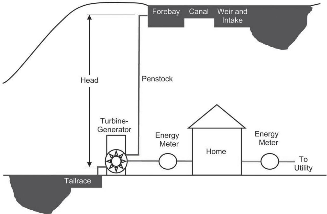
Figure - Grid-connected residential micro hydropower system. Meter between generator and home is optional.
